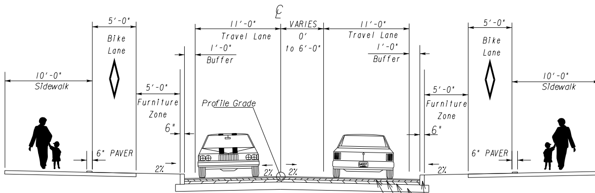
TYPICAL SECTION NO. 1 STA 10+12.58 TO STA 13+40.99
