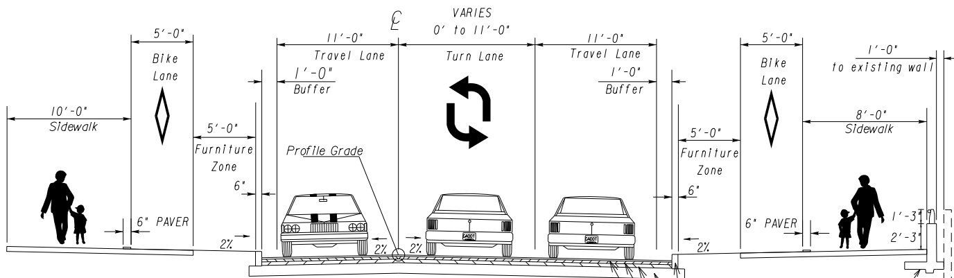
TYPICAL SECTION NO. 2 STA 13+40.99 TO STA 15+98.93 (PROPOSED RETAINING WALL STA 14+22.01 TO STA 15+82.01)
